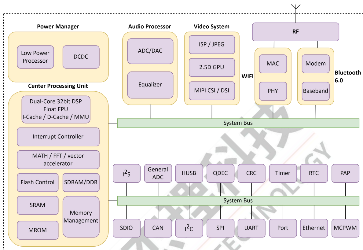
Figure 1-1 AC7922A Block Diagram
